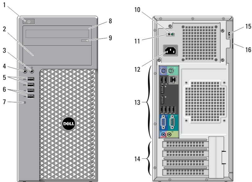
Figure 1. Front and Back View
