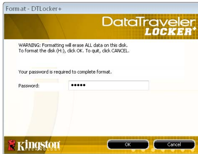
Figure 9: Format - DTLocker+
