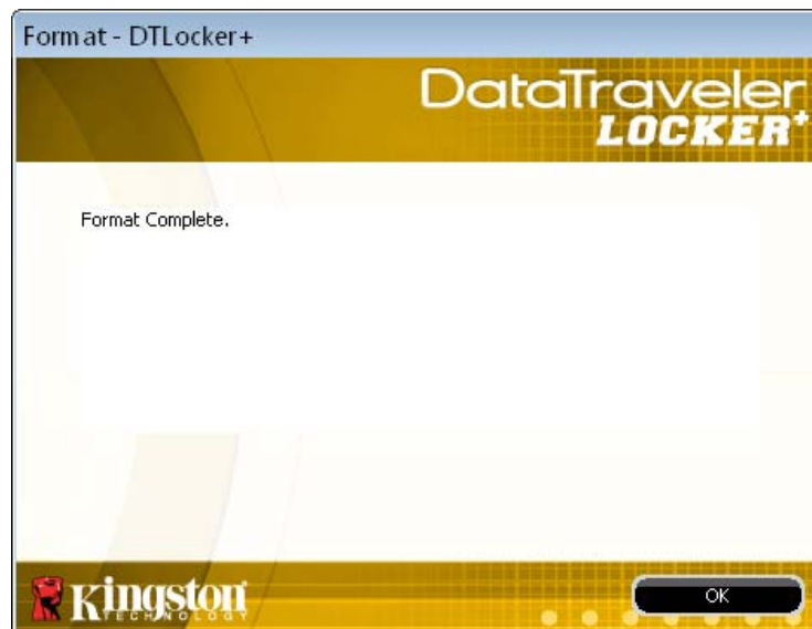
Figure 5: DTLocker+ Format
