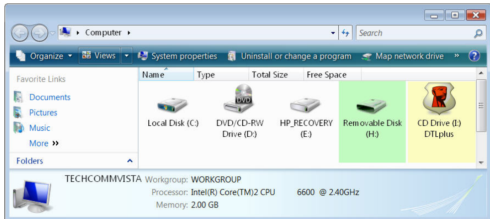
Figure 7: DTLocker+ Partitions
