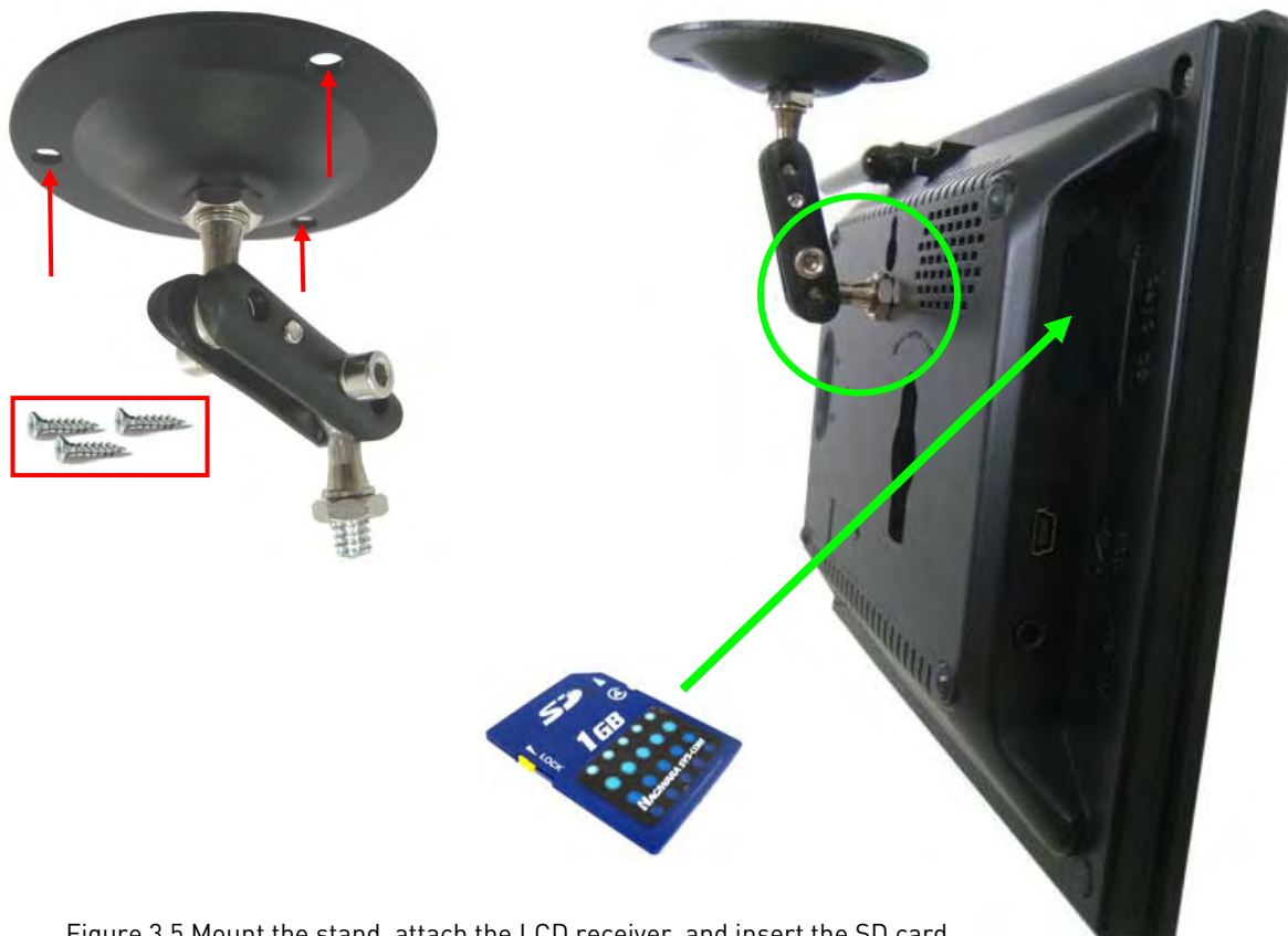
Figure 3.5 Mount the stand, attach the LCD receiver, and insert the SD card.
