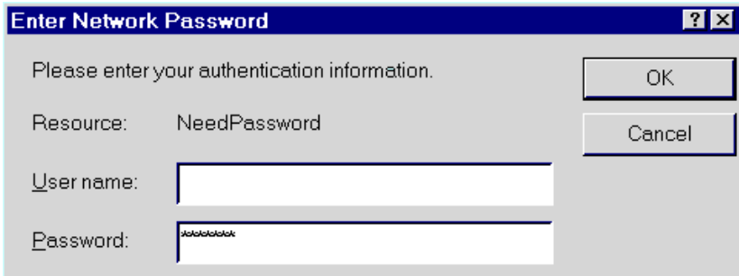
Figure 4: Password Dialog
