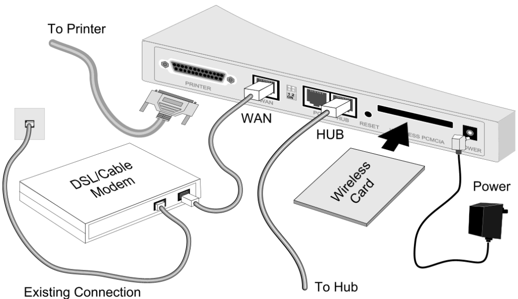
Figure 3: Installation Diagram
