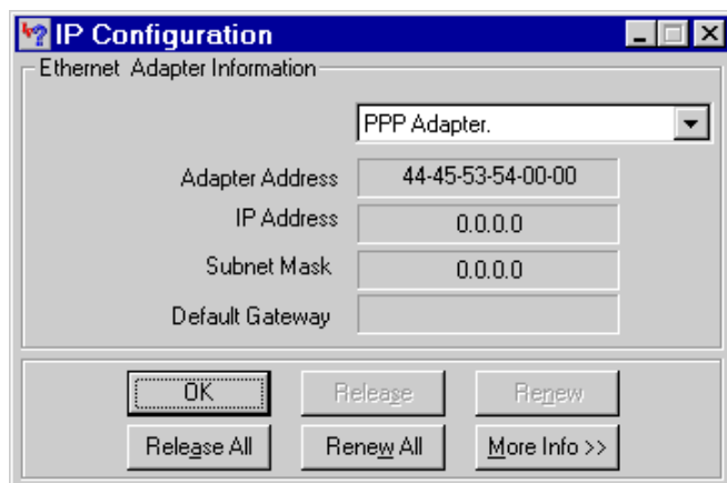
Figure 38: WinIpCfg
