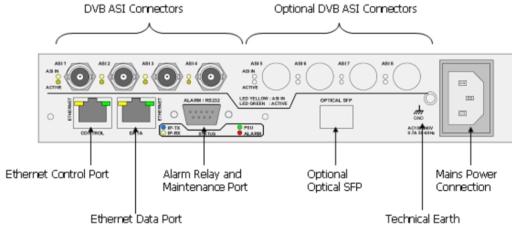
Figure 6. Rear panel connectors
