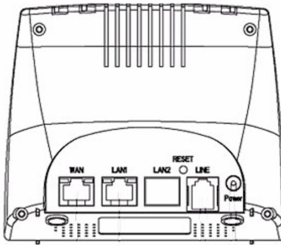
Rear Panel of VIP-321
