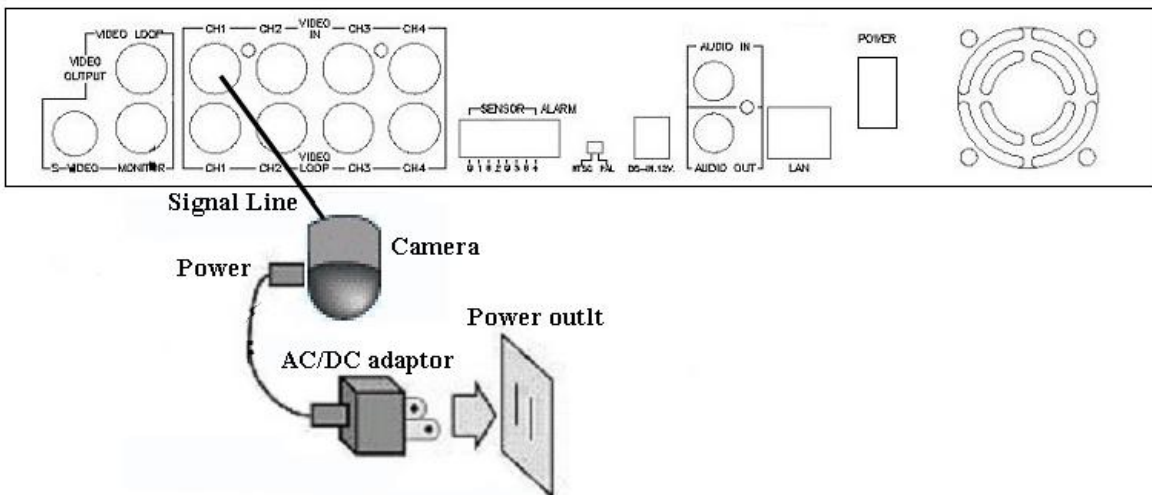
DVR-400 provides 4 x BNC connectors for video source input.
