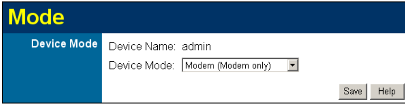
Figure 76: Mode Screen
