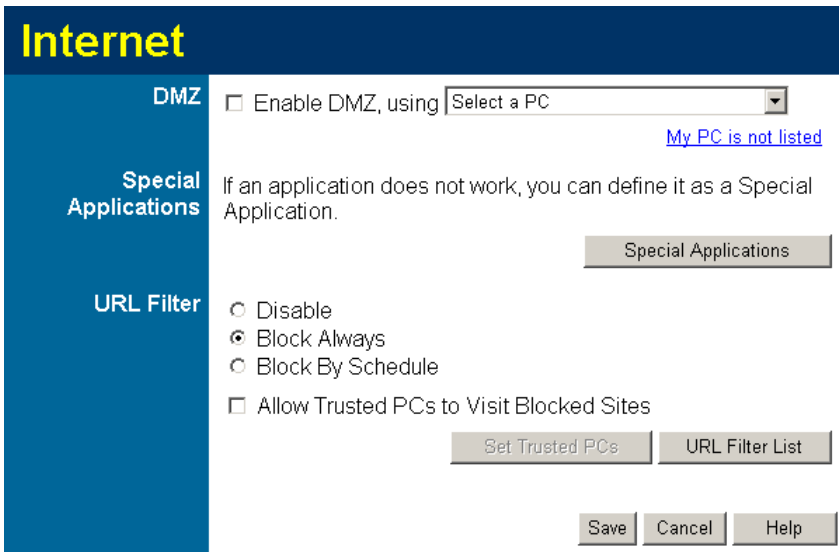
Figure 47: Internet Screen
