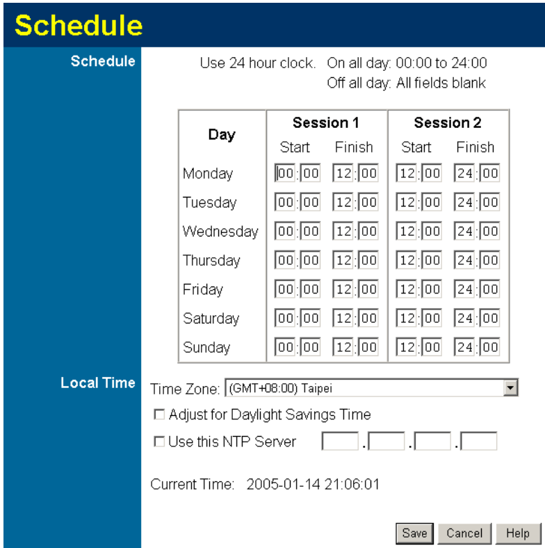
Figure 57: Schedule Screen
