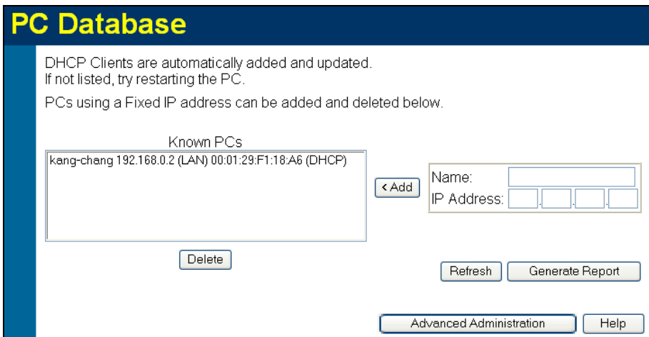
Figure 65: PC Database
