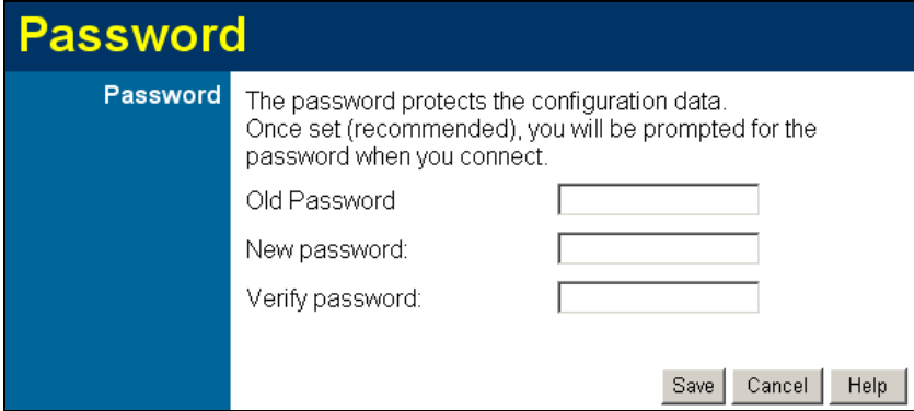
Figure 13: Password Screen
