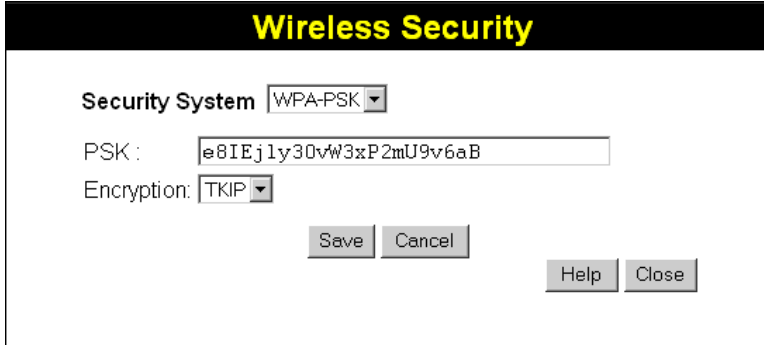
Figure 11: WPA-PSK
