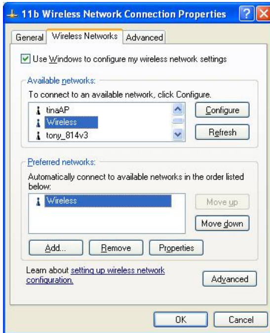
Figure 42: Preferred Networks
