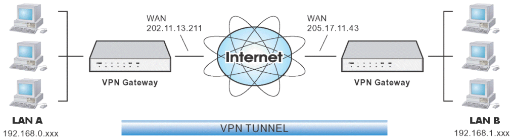
Figure 81: Connecting 2 ADE-4300/ADW-4300s
