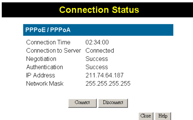
Figure 44: PPPoE Status Screen
