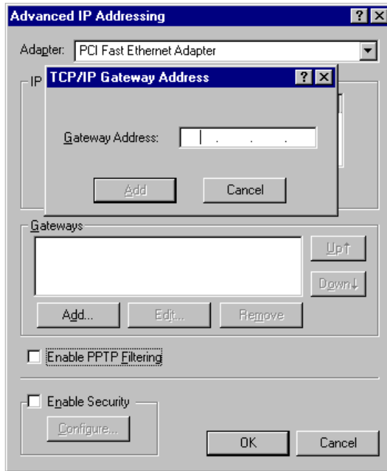
Figure 22 - Windows NT4.0 - Add Gateway
