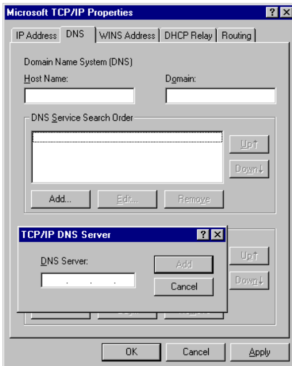
Figure 23: Windows NT4.0 - DNS
