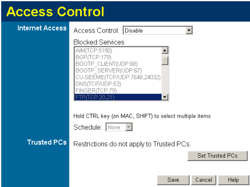
Figure 475: Access Control Screen
