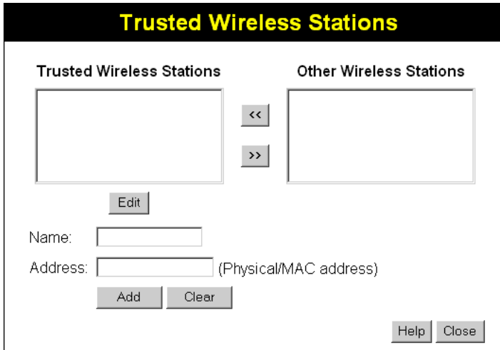
Figure 12: Trusted Wireless Stations
