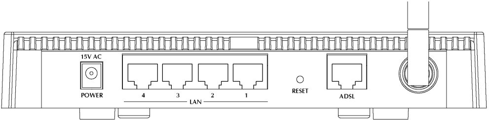
Figure 5-2: Rear Panel of ADW-4300
