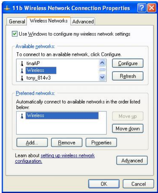
Figure 38: Preferred Networks
