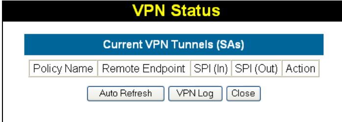
Figure 63: VPN-Status Screen
