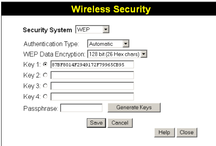
Figure 10: WEP
