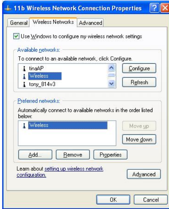
Figure 34: Preferred Networks
