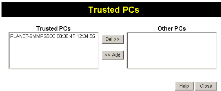
Figure 48: Trusted PCs
