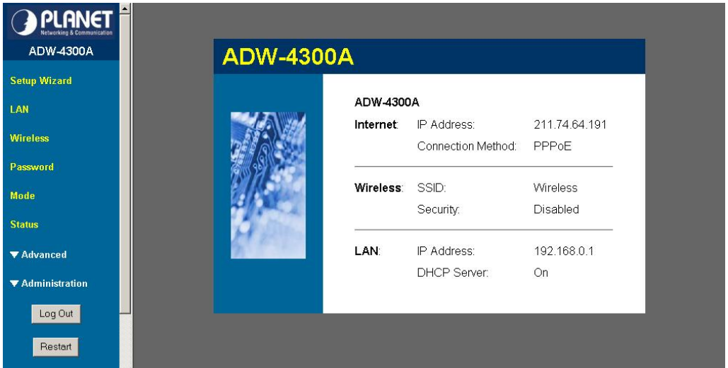
Figure 7: Home Screen
