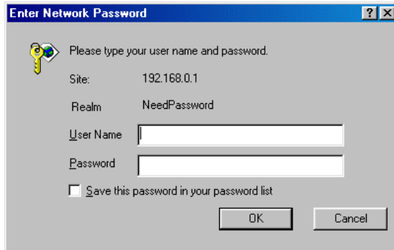
Figure 14: Password Dialog
