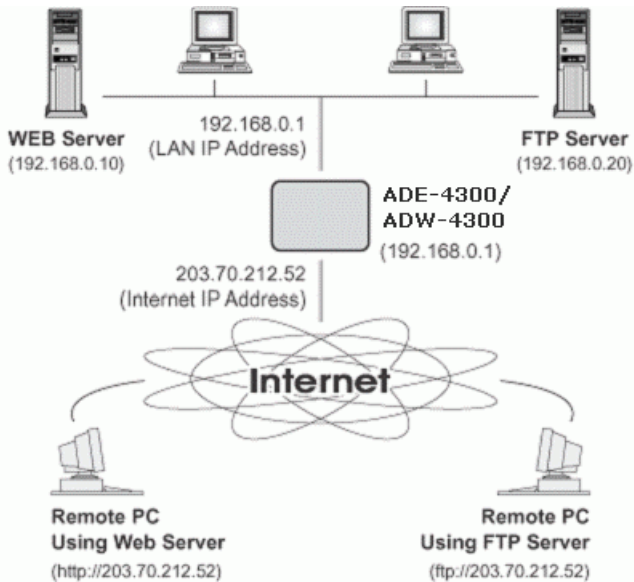
Figure 58: Virtual Servers
