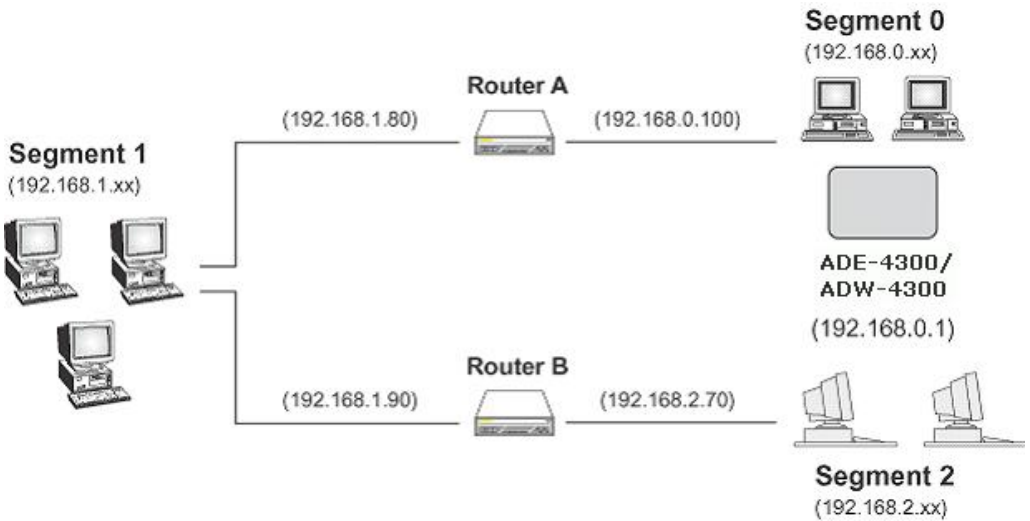
Figure 73: Routing Example
