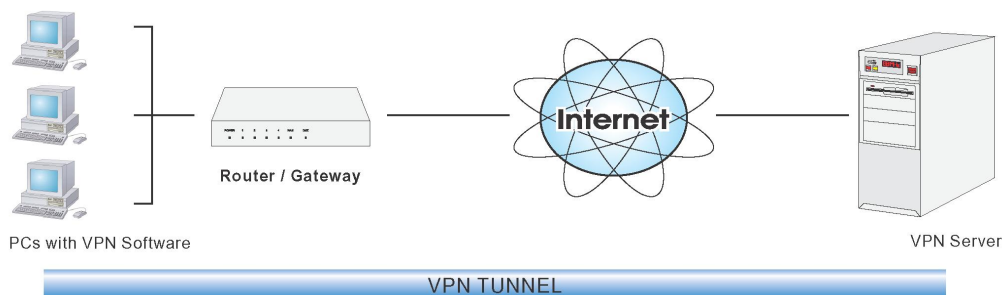
Figure 78: VPN Pass-through
