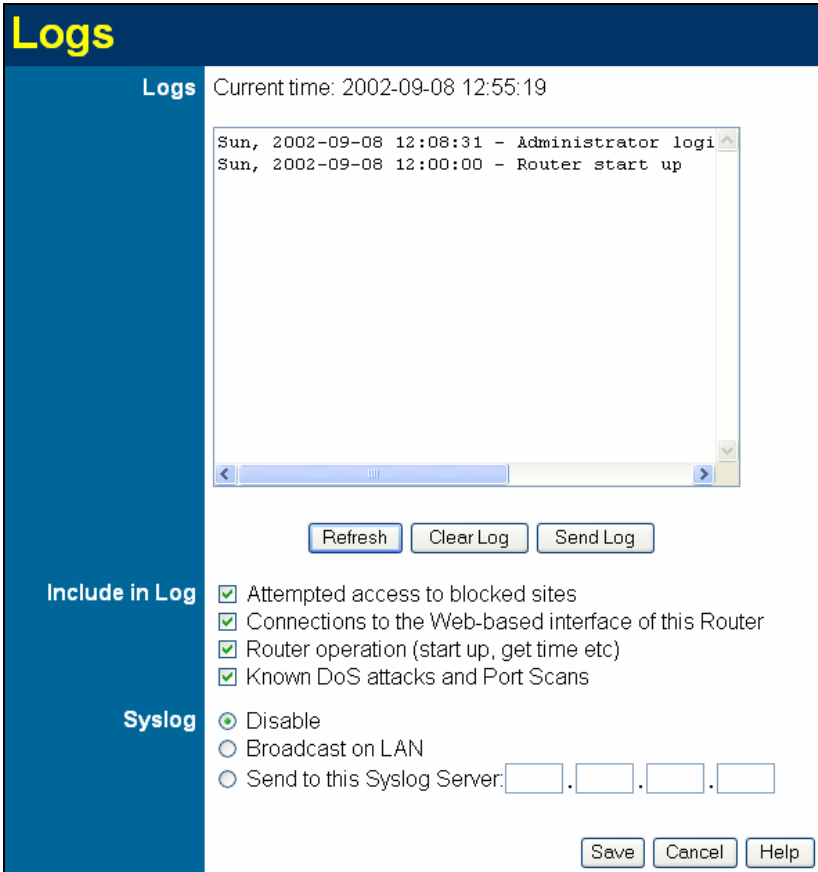
Figure 86: Logging Screen
