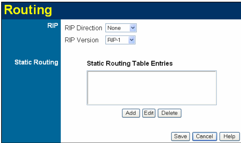
Figure 90: Routing Screen
