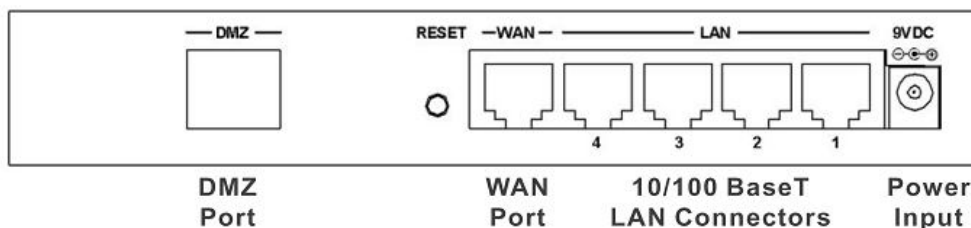
Figure 3: Rear Panel
