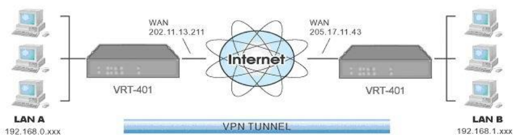
Figure 45: Connecting 2 VPN Gateways
