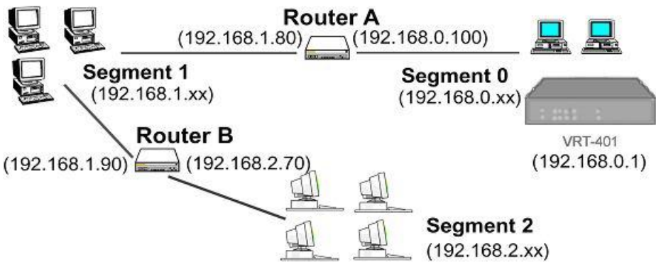
Figure 94: Routing Example
