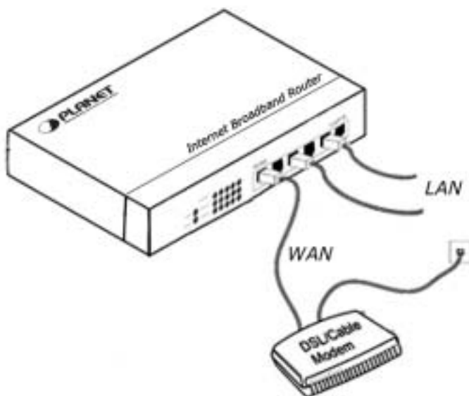
Figure 2-1: Installation Diagram
