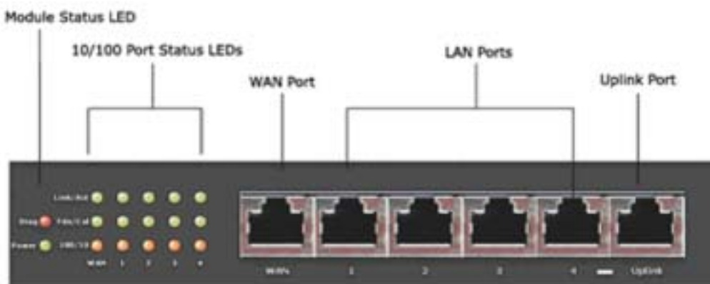
Figure 1-2: Front Panel
