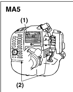
(1) Cylinder (2) Intake air cooling vent (back)
