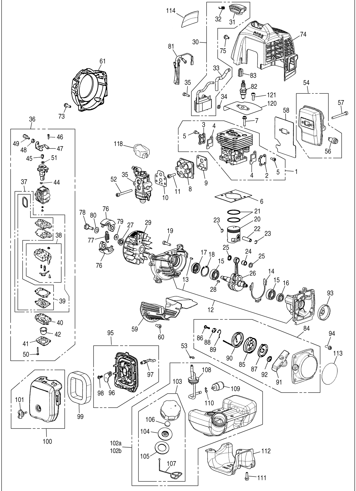
Fig.3 ENGINE UNIT (S/N 60100101 and up)
