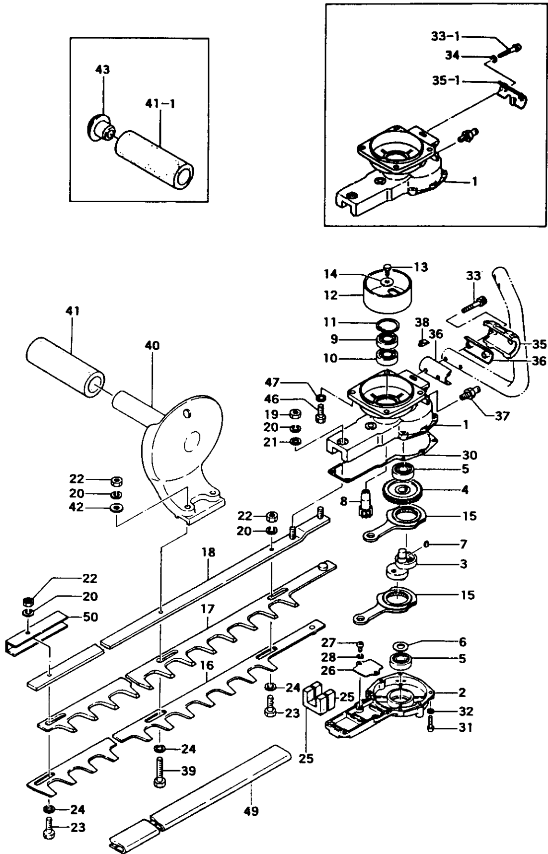
FIG.6 GEAR CASE & CUTTER
