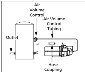
Figure 5 - Vertical Tank
