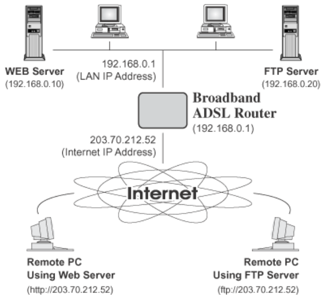
Figure 35: Virtual Servers
