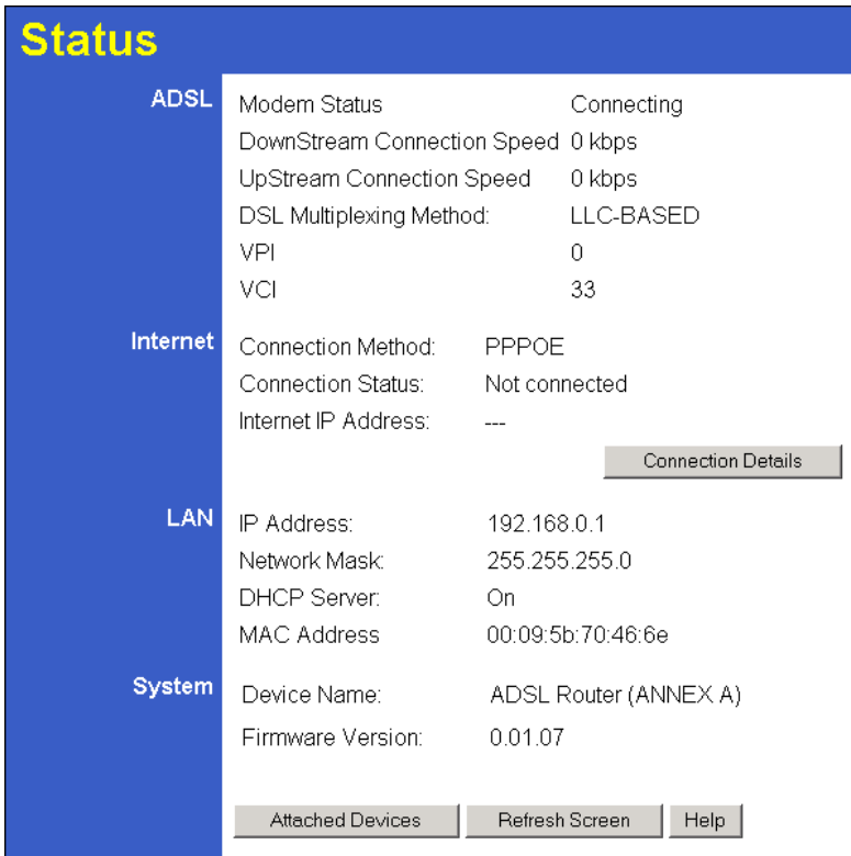
Figure 21: Status Screen
