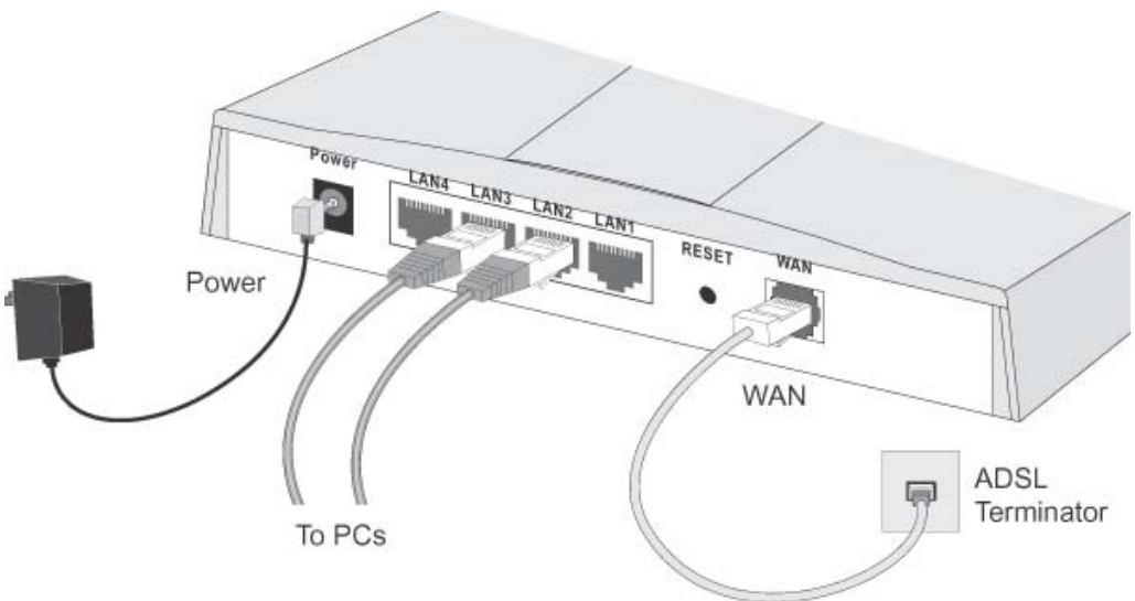
Figure 4: Installation Diagram
