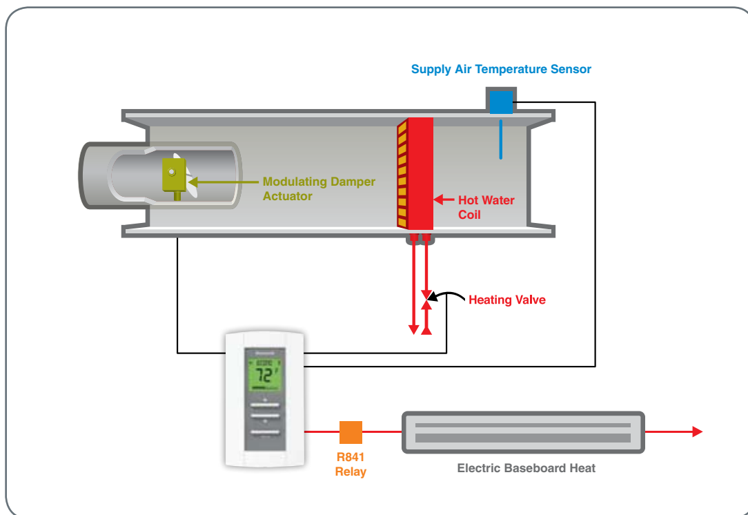
TB7980B1005: Cooling Only Pressure Dependent VAV Zone Reheat and Electric Baseboard Heat
