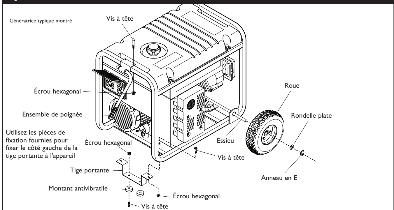
Figure 8 — Installe la roue la trousses
