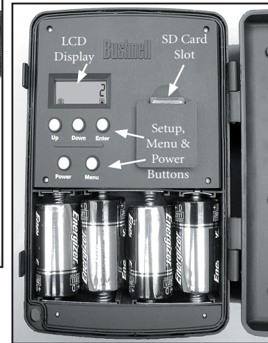
Control Panel Inside Front
