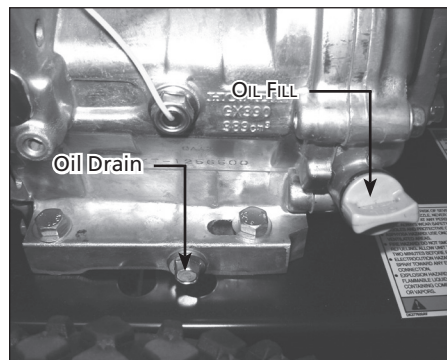
Figure 15 - Oil drain and fill locations
