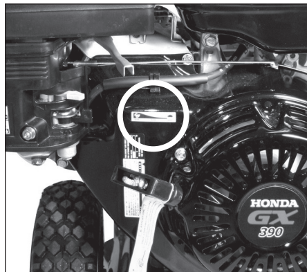
Figure 10 - Throttle
