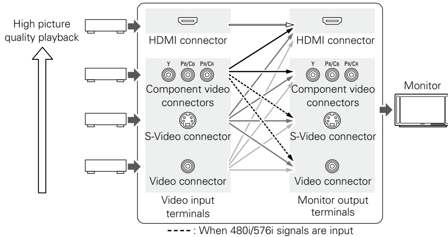
[Flow of video signals inside the AVR-2309]
