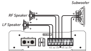
3 Channel Mode, 1 pair stereo plus one bridged channel
