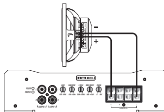
Mono Mode (This is the only configuration for this amplifier)
