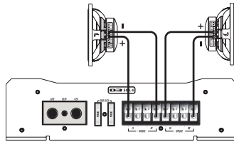
2 Channel Mode, both pairs of channels bridged
