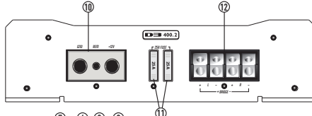
D3 400.2 2-Channel Amplifier
