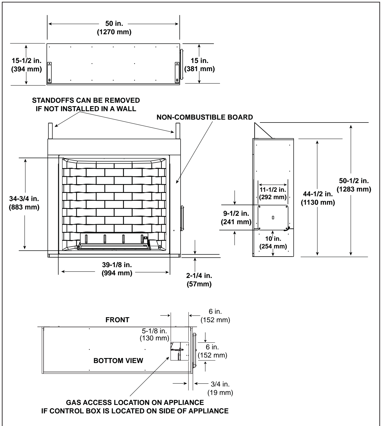
Figure 12.2 Appliance Dimensions - CARODG42I, CARODG42IL
