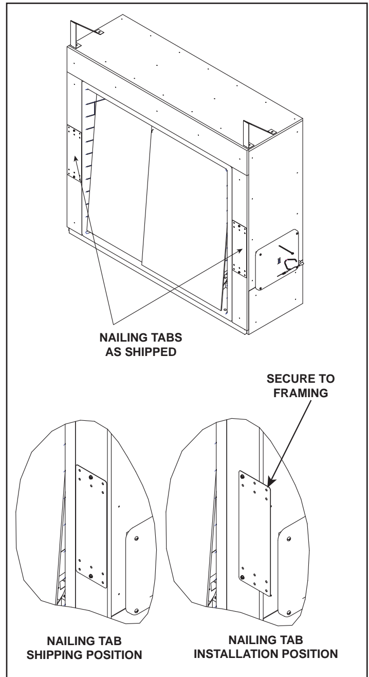
Figure 4.1 Positioning and Securing Nailing Tab
