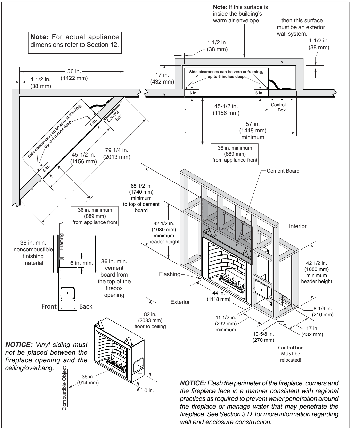
➔ Figure 3.1 Appliance Locations and Framing Dimensions - CARODG36I, CARODG36IL
