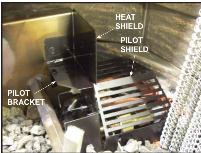
Figure 8.1 Pilot Shield Position
