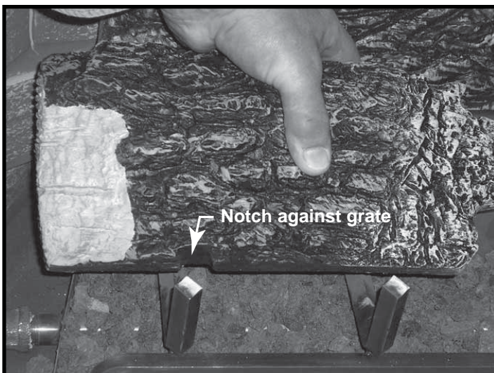
Figure 8.5 Place Left Front Log
