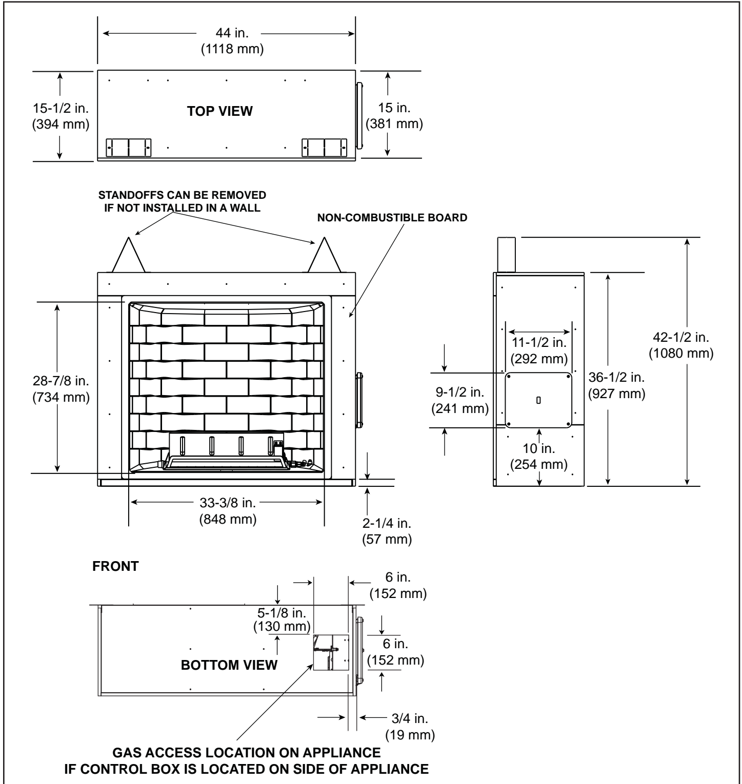
Figure 12.1 Appliance Dimensions - CARODG36I, CARODG36IL
