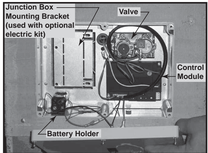
Figure 5.3 Control Box
