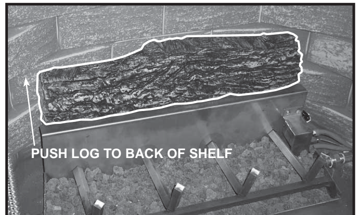
Figure 8.4 Place Rear Log - Carolina-36
