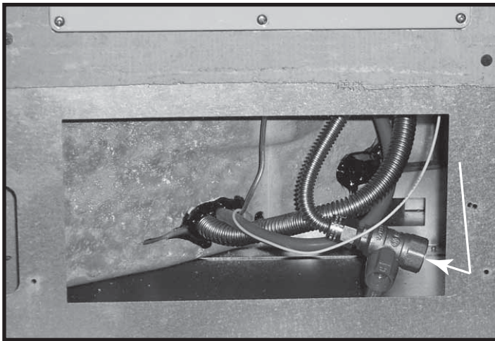
Figure 5.2 Connect Incoming Gas Line to Manual Shutoff Valve
